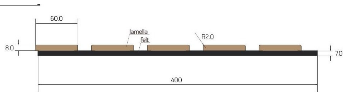
Technical drawing
